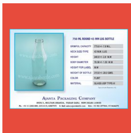
750 MI Juice Bottle
