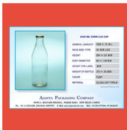
1000 ML Milk, Juice, Water Glass Bottle
