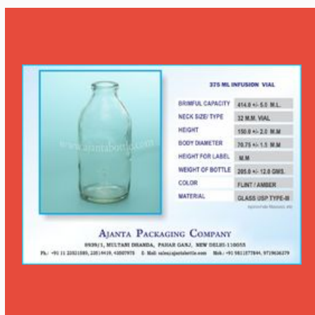
375 ML Infusion Vial
