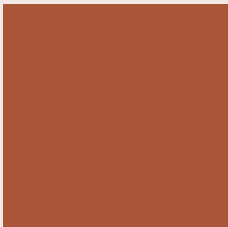
2,4-Dinitrophenyl Hydrazine
