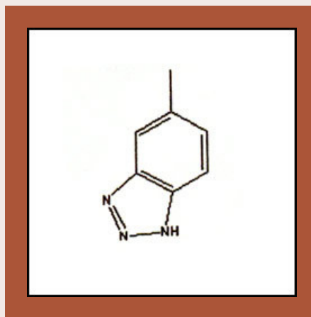
5-Methyl-1H-Benzotriazole
