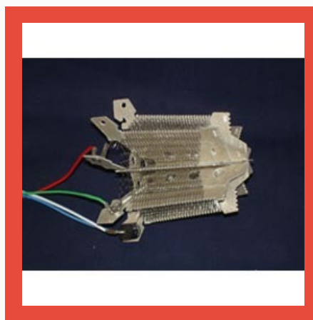
Mica Heater for Hair Dryers
