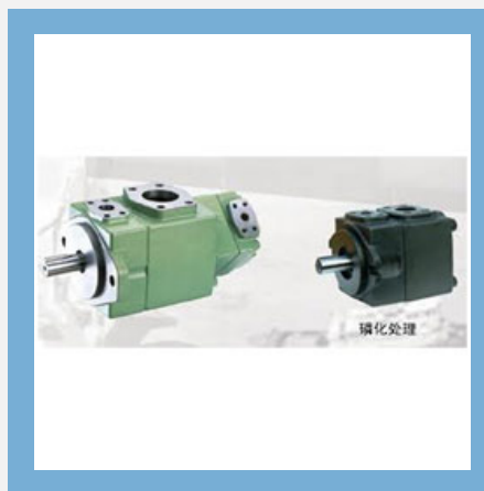
Fixed Displacement Vane Pumps
