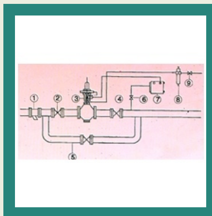
Automatic Pressure Reducing Station
