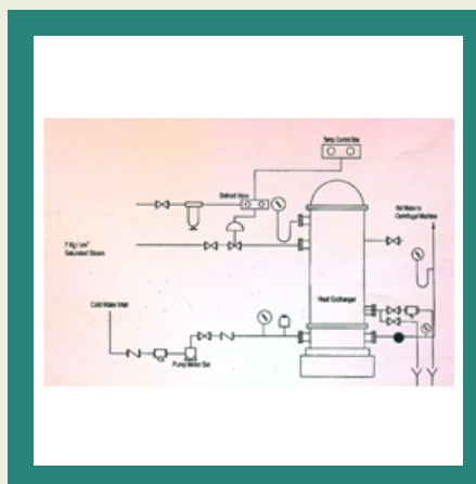
Superheated Wash Water System
