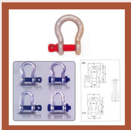
Forged Shackles
