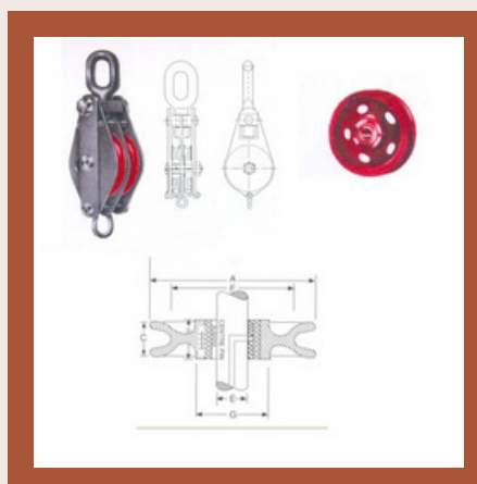
Double Sheave Pulley Block
